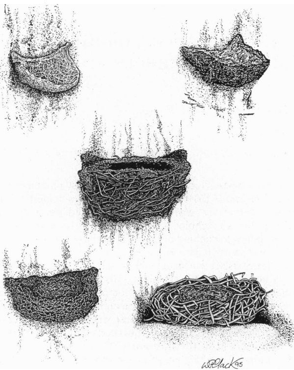
FIG. 1. Swiftlet nests showing species-specific variation in characters used for swiftlet taxonomy. Illustrations are of voucher nests collected from populations also sampled for DNA work. (Upper Left) A. fuciphagus vestitus nest made entirely of, and vertically supported by, salivary "glue" ( A. fuciphagus is the only species with a pure saliva nest). (Upper Right) A. maximus nest made of saliva and feathers and vertically supported. (Middle) A. brevirostris nest made of saliva, feathers, and vegetation and vertically supported. (Lower Left) A. spodiopygius assimilis nest made of saliva and vegetation and vertically supported. (Lower Right) A. sawtelli nest made of saliva and vegetation and supported by a horizontal surface.
